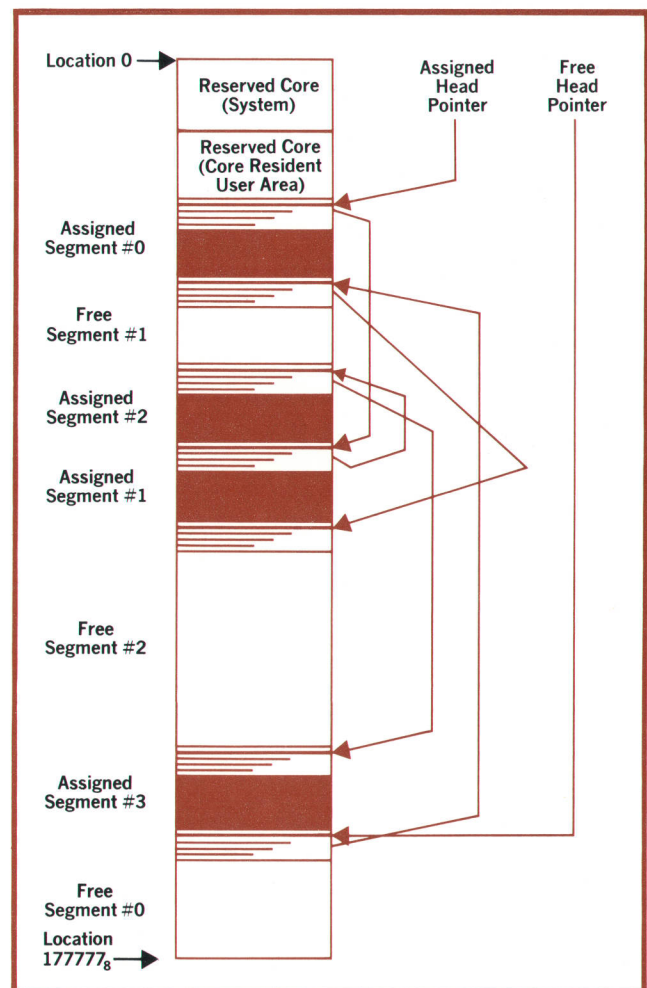
Fig. 2 Main memory is organized into reserved and linked memory. Linked memory consists of free and assigned areas.
